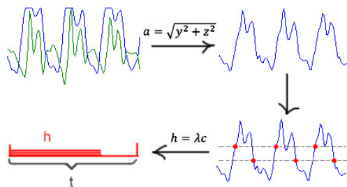
Figure 2: Algorithm of calculating running time.
